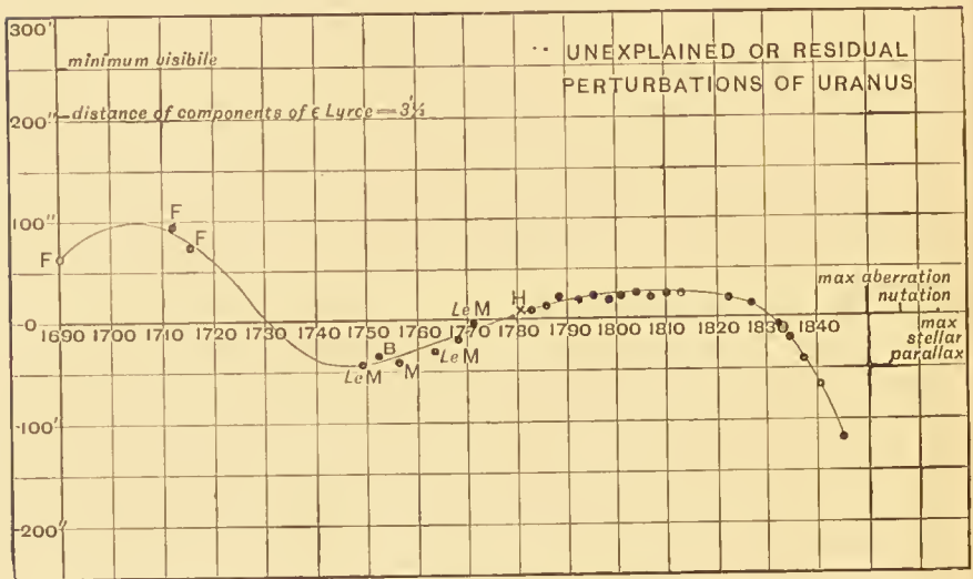
FIG. 93.—Perturbations of Uranus.
